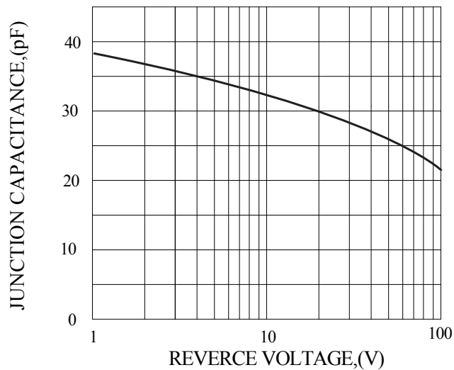
FIG.5-TYPICAL JUNCTION CAPAOTANCE
