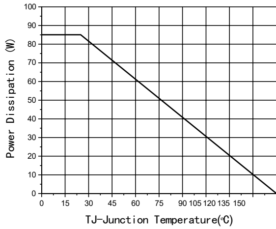
Fig7 Power De-rating
