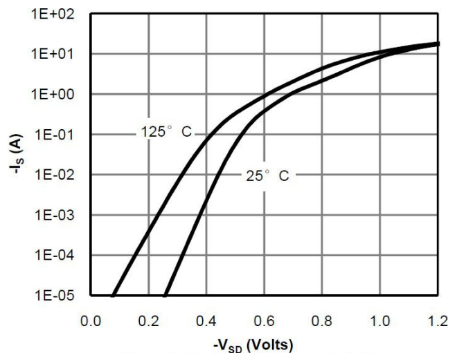
Figure 6: Body-Diode Characteristics
