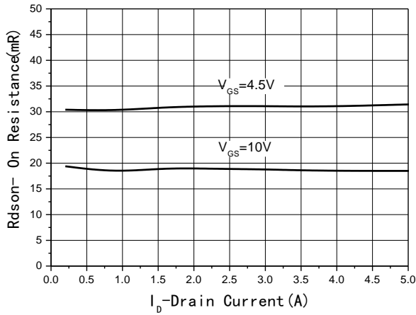
Fig3 Rds(on)-Drain current
