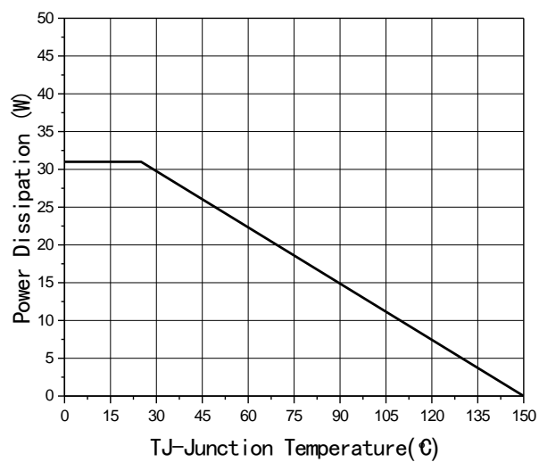
Fig7 Power De-rating
