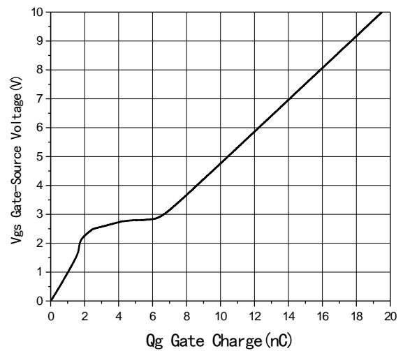
Fig6 Gate Charge
