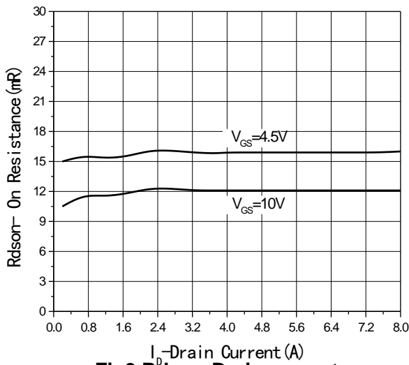
Fig3 Rds(on)-Drain current
